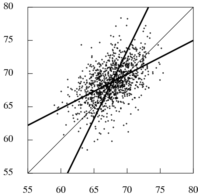
Figure 1. Pearson’s data comprising 1078 measurements of the heights of fathers (the abscissae) and of their sons (the ordinates), together with the two regression lines. The correlation coefficient is 0.5013.
