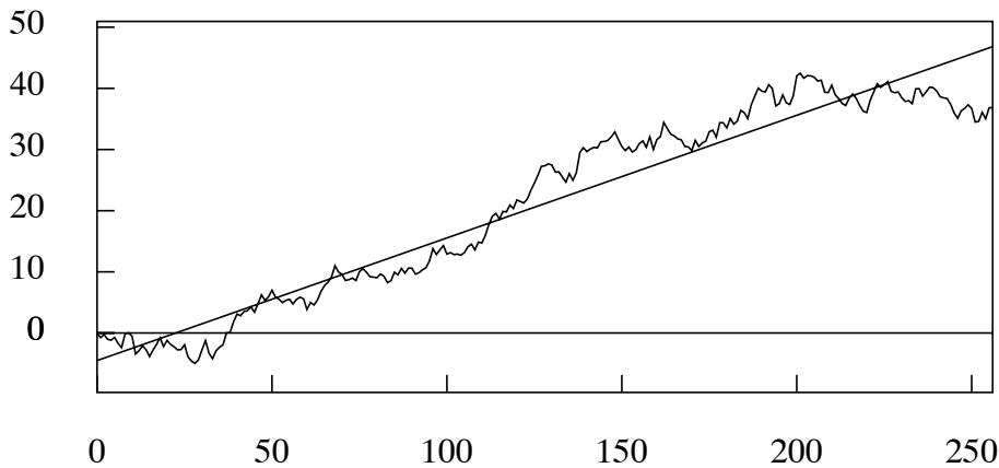
Figure 2. A random walk generated by the equation y_t = y_{t-1} + \alpha + \varepsilon_t together with an interpolated regression line. The variance of the white-noise disturbance is V(\varepsilon_t) = 1 and the drift parameter is \alpha = 0.2 .
