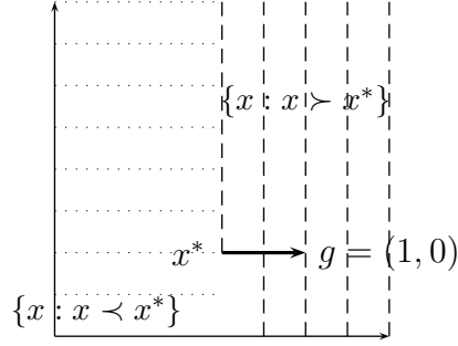
Figure 1: Lexicographic order
