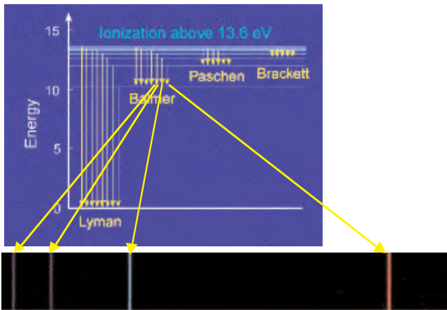
Figure 3. (Top) Energy level diagram of the hydrogen atom, showing some of the possible transitions that can take place between levels. (Bottom) The distinctive pattern of the hydrogen emission lines some possible transitions and an example spectrum are shown in figure 3. The more complex the atom (i.e. the more electrons it has), the more energy levels are available and, therefore, a greater variety of transitions can take place. So, while we see only a few spectral lines associated with hydrogen, we see many more for complex atoms such as iron. These patterns of lines are a unique “cosmic fingerprint”, from which we can identify each element.
