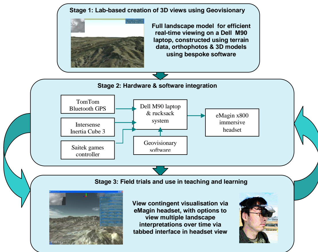
Figure 5. Augmented reality system for field teaching based on Geovisionary software
