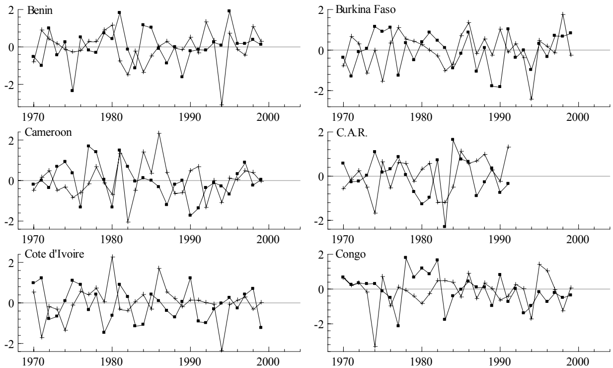
Figure 3: \varepsilon_{it}^P (+) and \varepsilon_{it}^Y (■) time series
