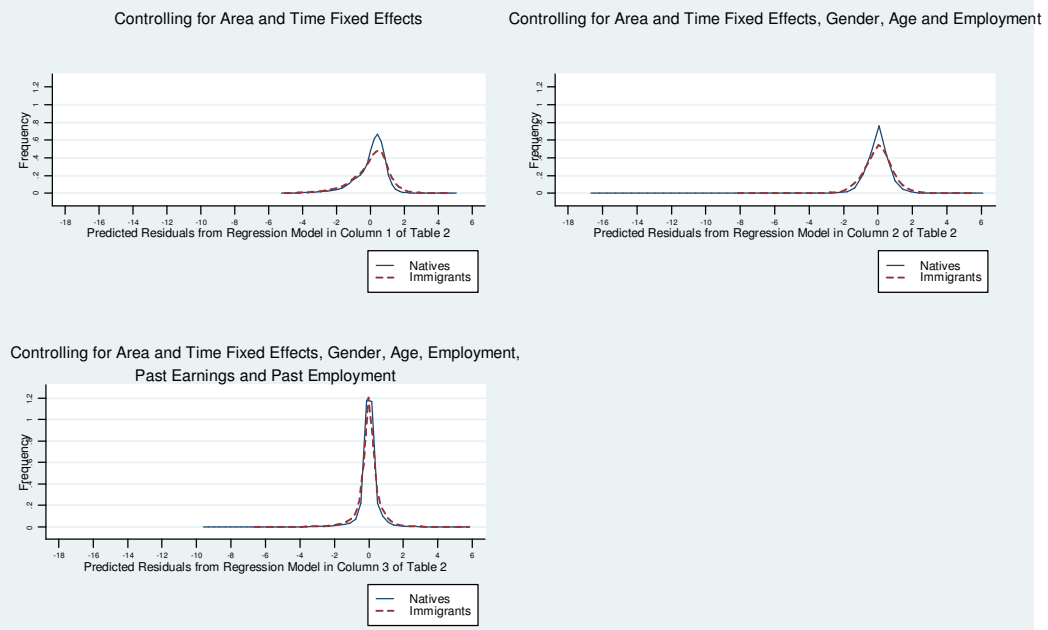
Figure 8 - Predicted Residuals
